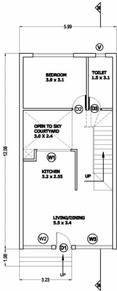
TYPICAL GROUND FLOOR PLAN (D1 & D8)
