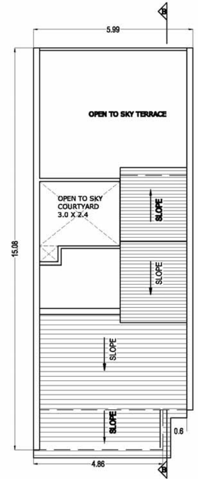
TYPICAL ROOF PLAN (D1 & D8)
