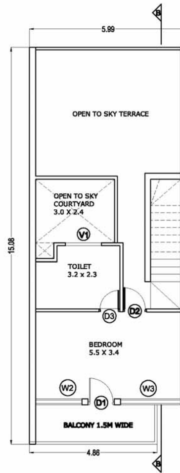
TYPICAL SECOND FLOOR PLAN (D1 & D8)
