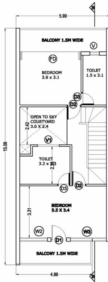
TYPICAL FIRST FLOOR PLAN (D1 & D8)
